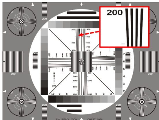
Figure 1: EIA-1956 Test Chart with enlarged portion at upper right
