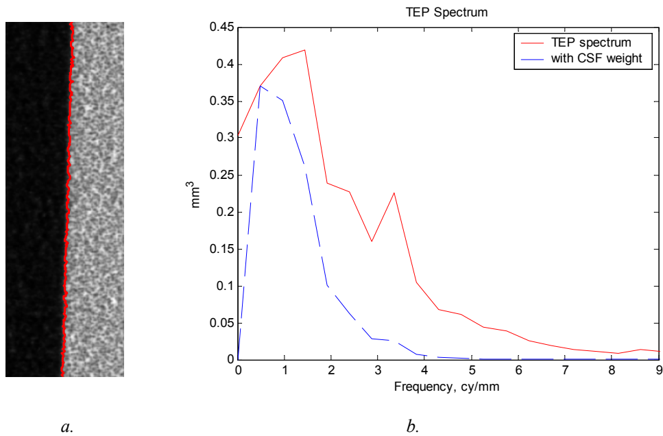
Figure 6: (a) Scanned inkjet print with detected edge added, and (b) TEP noise-power spectrum and CSF weighting for 33 cm viewing distance.
