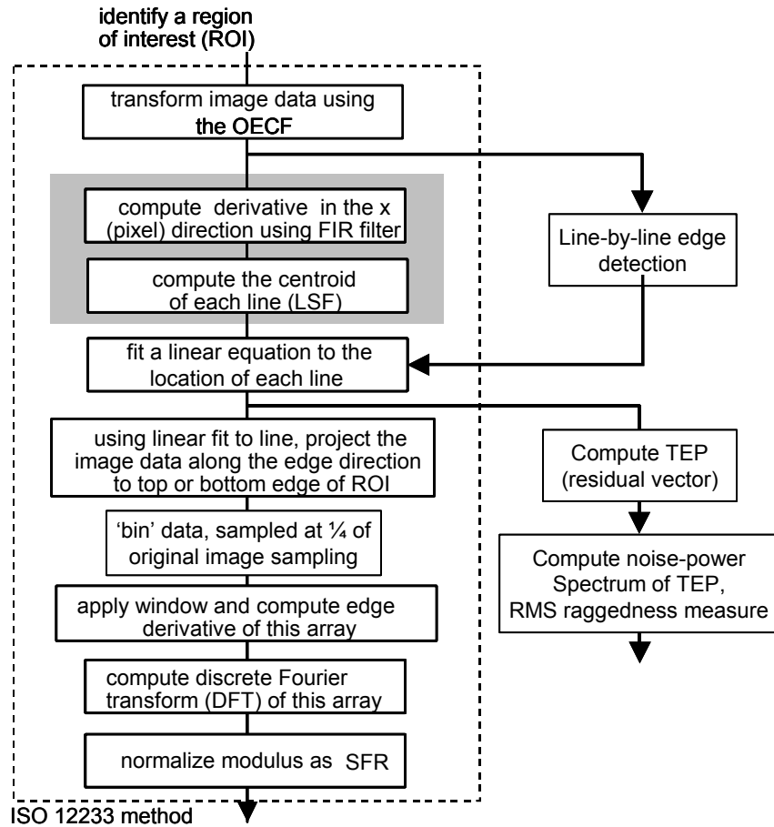
Figure 3: Outline of the slanted-edge analysis method (left-hand side), with additions for raggedness evaluation on the right. The sampled edge is assumed to be near vertical.
