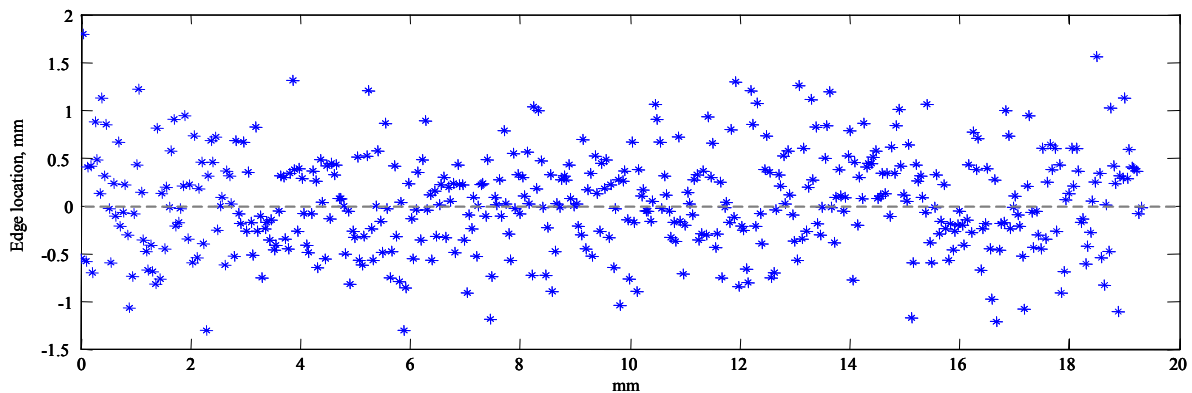
Figure 4: Example TEP for an electrophotographic printed edge
