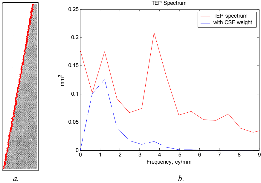
Figure 5: (a) Scanned electrophotographic print with detected edge added, and (b) TEP noise-power spectrum and CSF weighting for 33 cm viewing distance.
