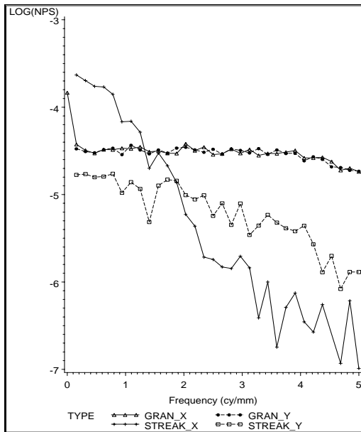
Figure 3. Streaking and Granularity NPS for Synthetic Pattern
