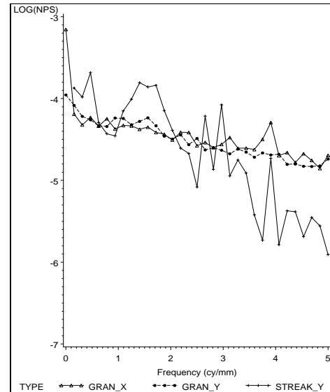
Figure 6. Streaking and Granularity NPS for Digital Printer Flat Field
