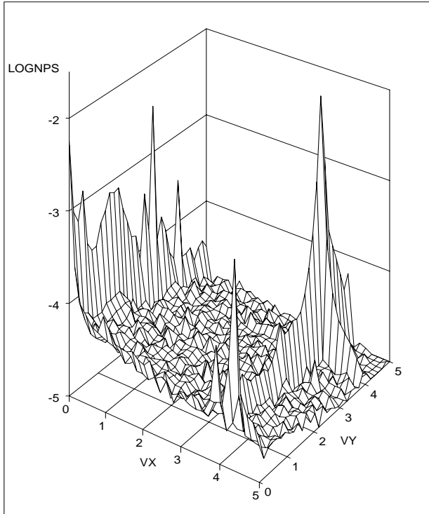
Figure 5. Two-dimensional NPS of Digital Printer Flat Field.
