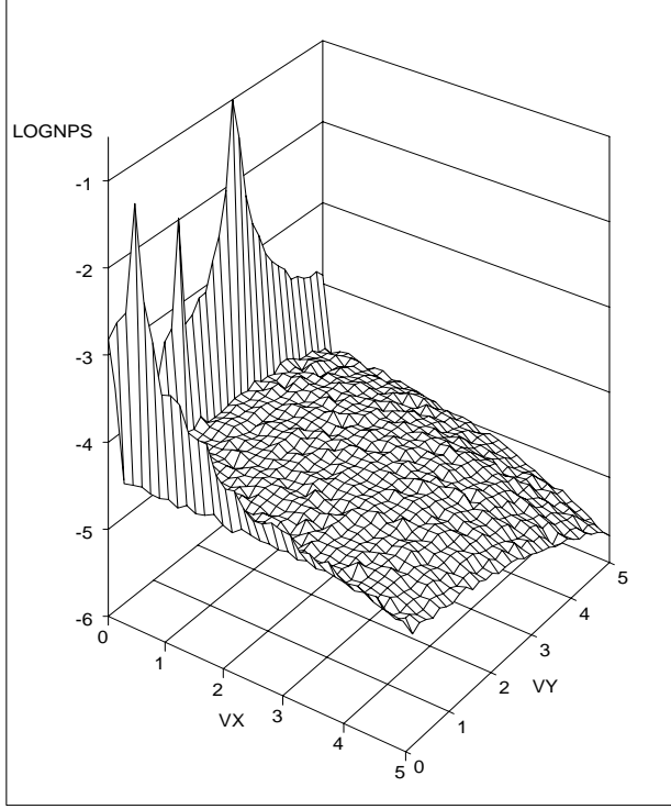
Figure 2. Two-dimensional NPS of Synthetic Pattern. The frequency axes are [0-5 cy/mm].
